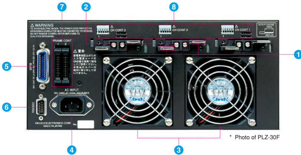
Rear panel
