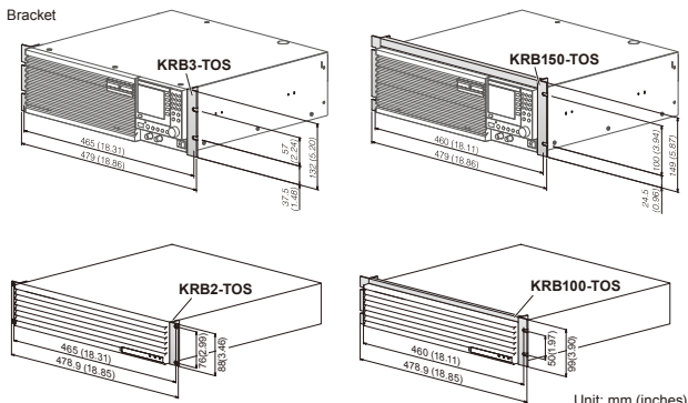
Bracket
