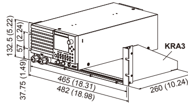
for EIA-compliant rack KRA3
