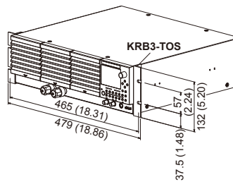
for EIA-compliant rack KRB3-TOS
