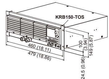
for JIS-compliant rack KRB150-TOS
